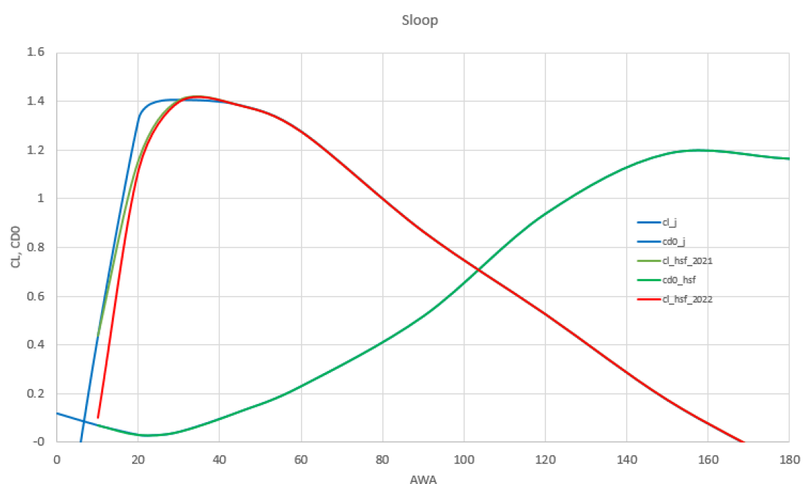
Figure 3: example of global lift-drag coefficients of luffed headsails (cyan) vs. flying headsails (green), sloop rig. The red line shows the Cl coefficients as modified in 2022
