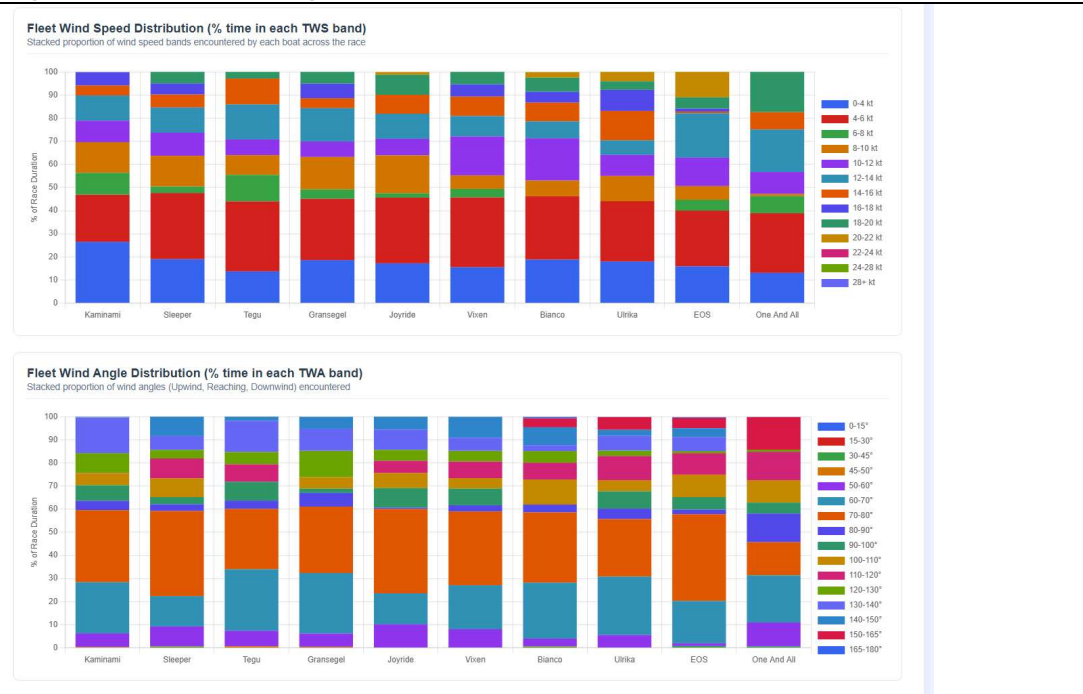
Figure 7. TWS and TWA angle distribution for the fleet.
