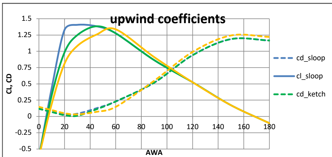
Figure 2: upwind aerodynamic coefficients.
