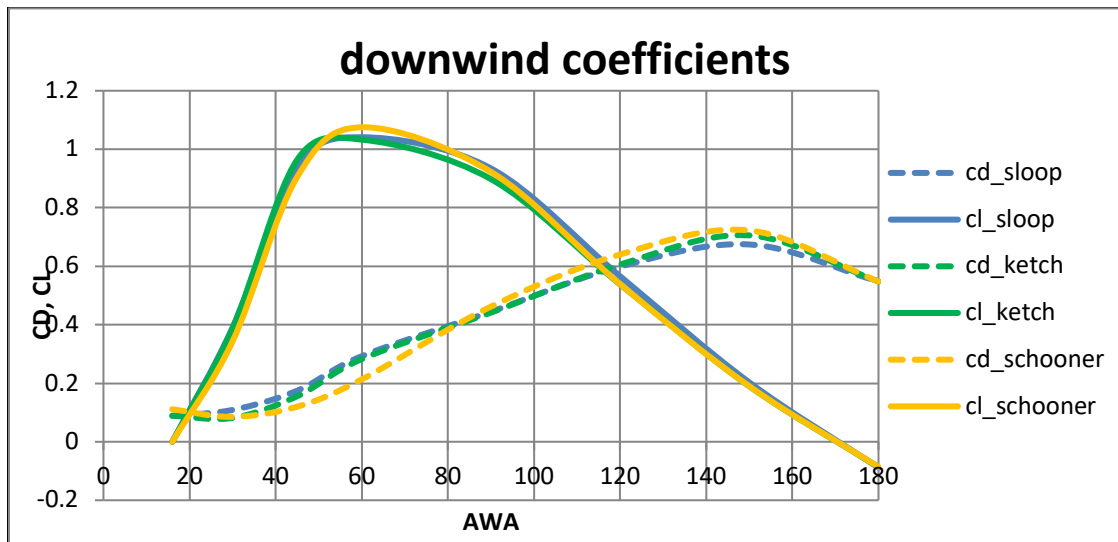
Figure 3: downwind aerodynamic coefficients.
