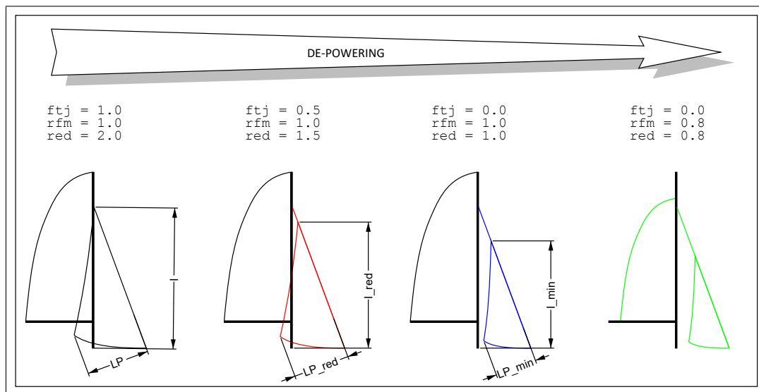
FIGURE 5.3: De-powering scheme
