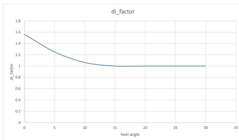
FIGURE 6.10: Multiplier of induced drag
