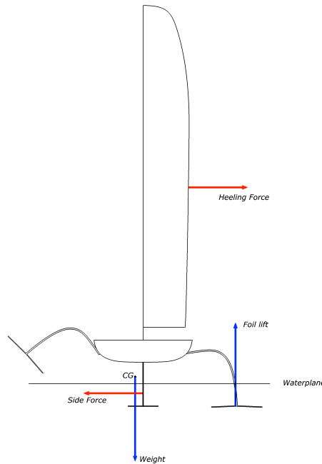
FIGURE 3.7: Equilibrium scheme for full foiling yacht
