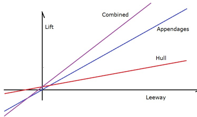
FIGURE 6.9: Induced Drag
