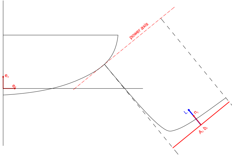
FIGURE 3.6: Foil power axis, area and span definition
