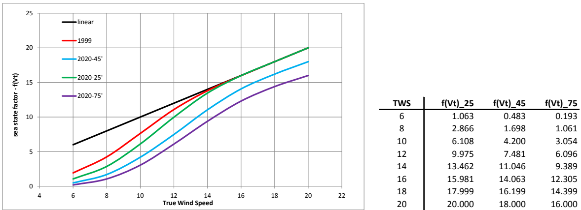
FIGURE 6.14: Wave Energy as a function of True Wind Velocity
