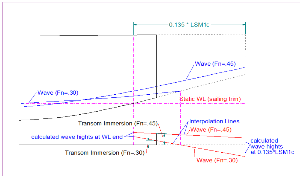
FIGURE 6.13: Principle of estimating transom immersion
