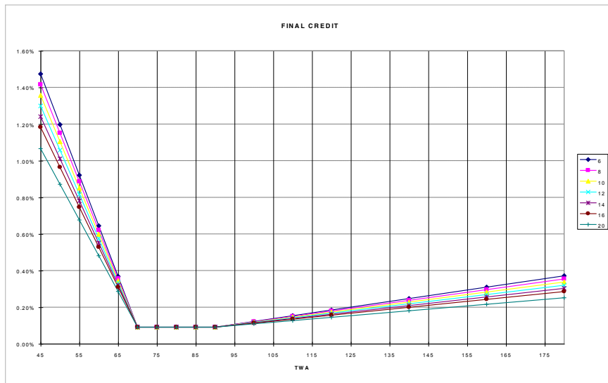
FIGURE 3.8: DA credit vs. True Wind Angle.
