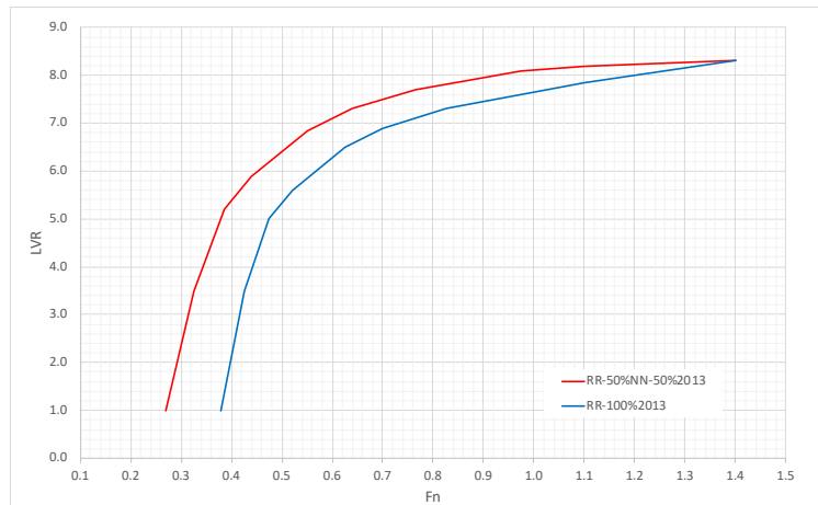
FIGURE 6.7: LVR-Fn boundaries of RR blending zone
