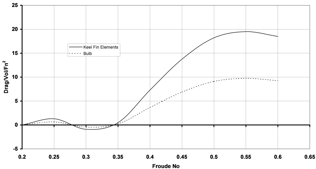
FIGURE 6.8: Appendage residuary resistance per unit volume at standard depth.
