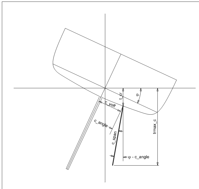
FIGURE 6.11: Scheme of bilgeboards and related variables
