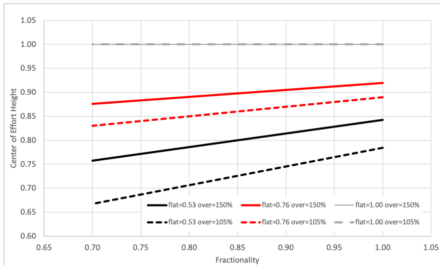
FIGURE 5.14: Twist Function
