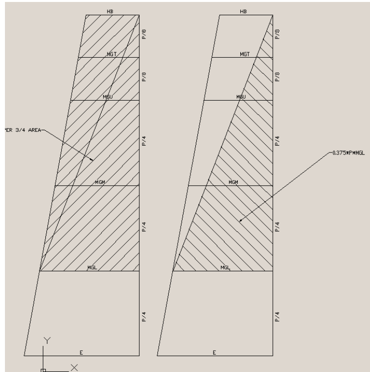
FIGURE 5.5: Roach calculation
