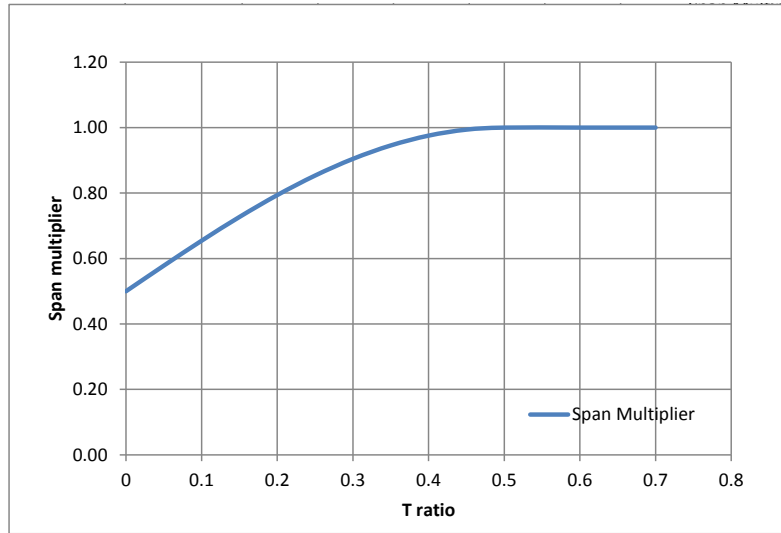
FIGURE 6.12: Keel root free surface factor
