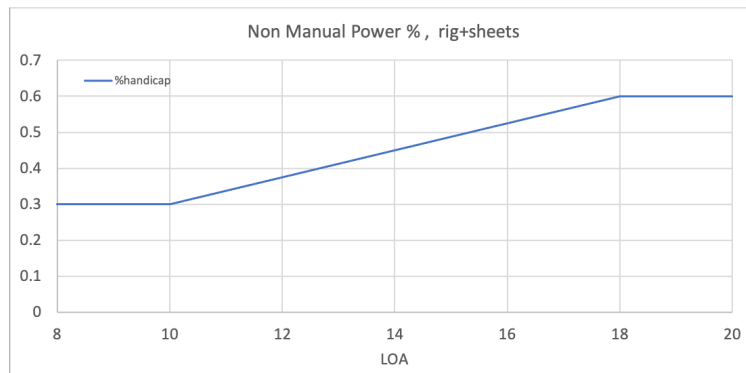
FIGURE 3.9: Max penalty for non manual power as function of overall length.
