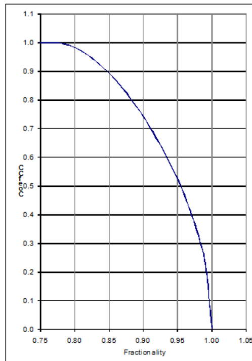
FIGURE 5.7: Fractionality Coefficient
