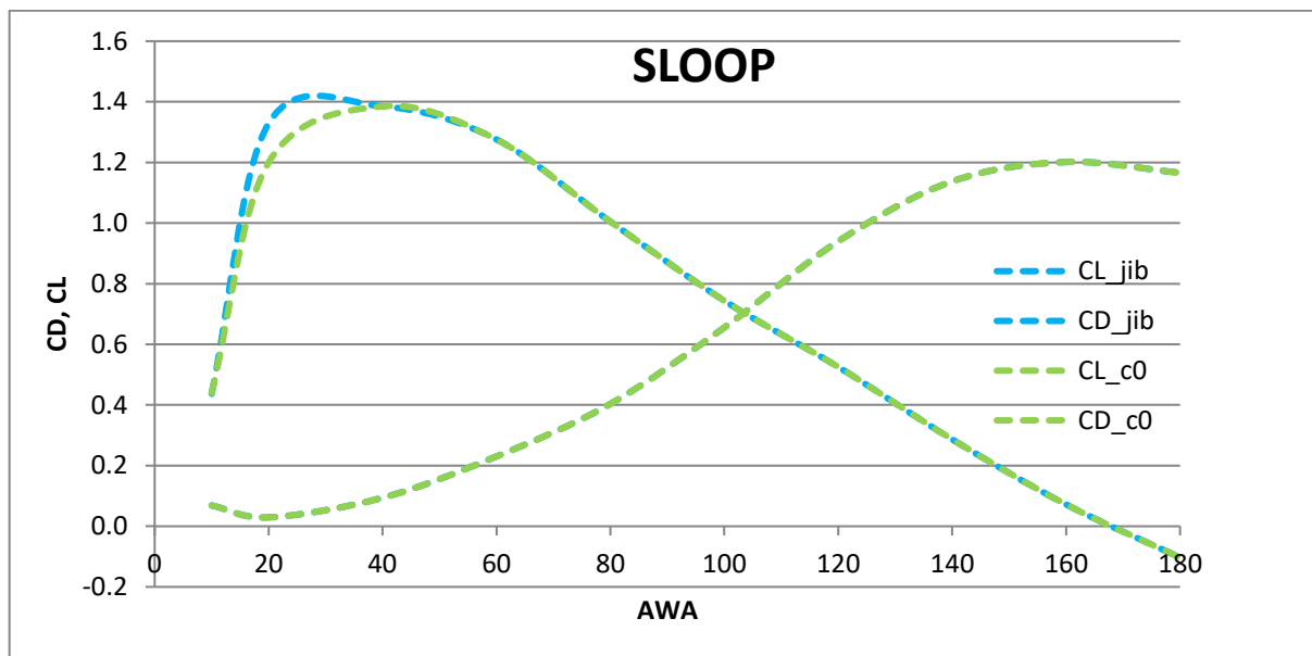
Figure3: example of global lift-drag coefficients of luffed headsails (cyan) vs. flying headsails (green), sloop rig.
