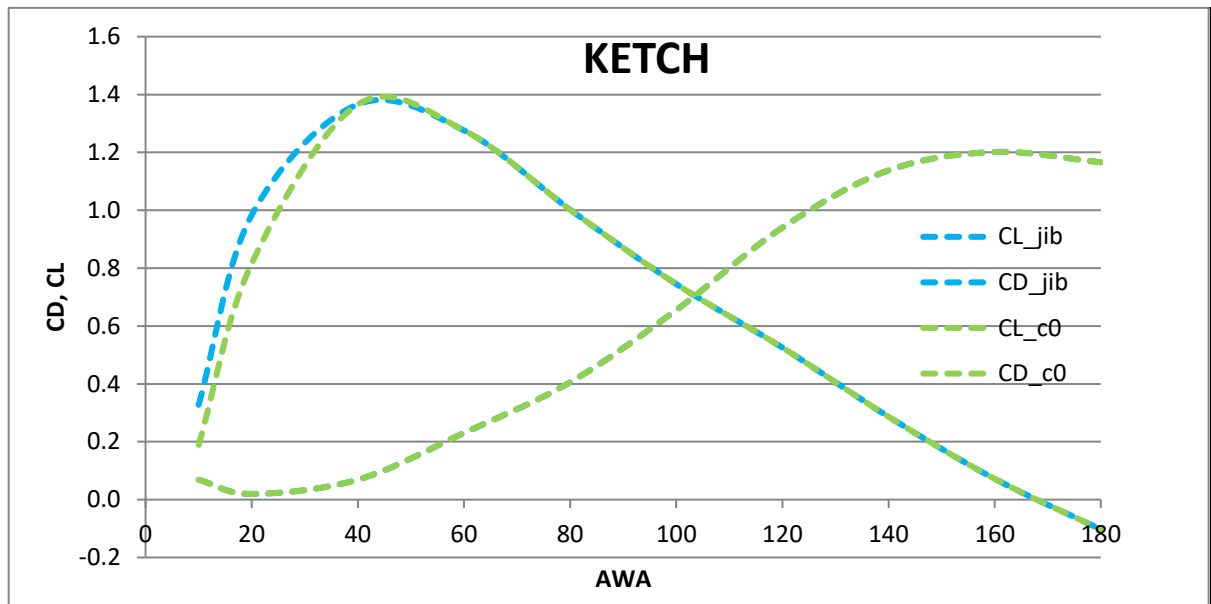
Figure4: example of global lift-drag coefficients of luffed headsails (cyan) vs. flying headsails (green), ketch rig.
