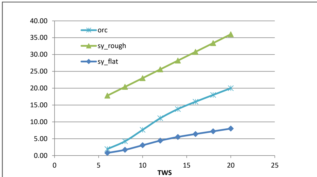
Figure 1. ORC and SY true wind speed behavior of the added resistance in waves.
