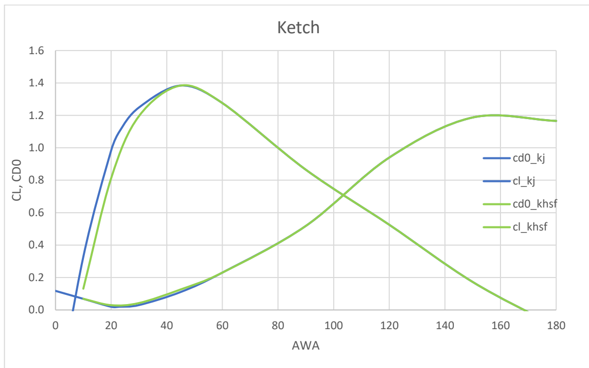
Figure4: example of global lift-drag coefficients of luffed headsails (cyan) vs. flying headsails (green), ketch rig.
